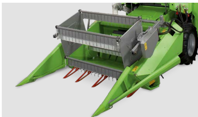
Header with feeding auger and feeder house
